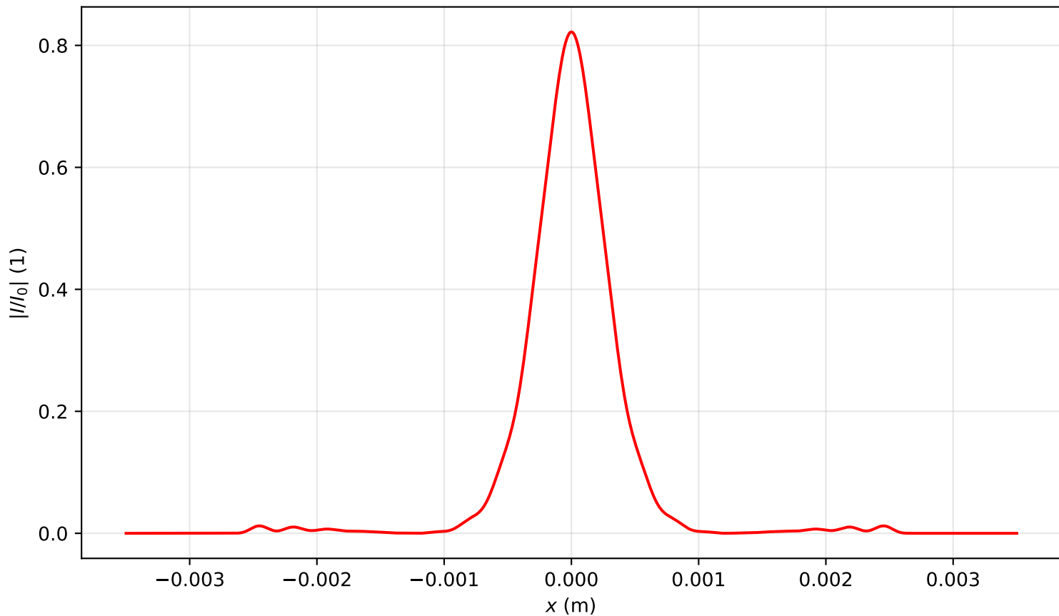
Intensity profile I(x, y = 0, z = 1.751)/I_0 , P_{in}=1.0P_{cr} , artificial time
